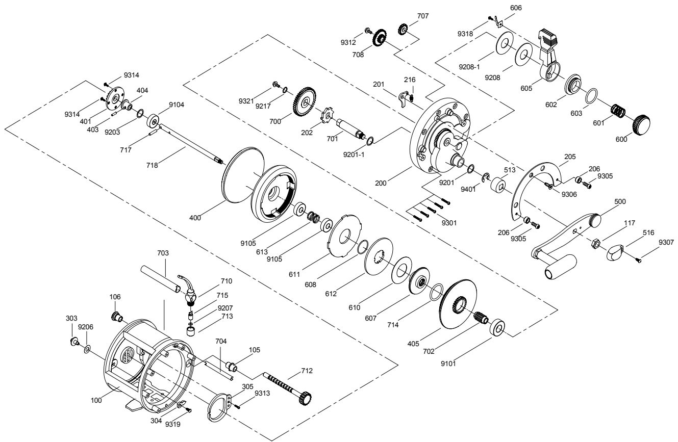
T - 15L Spare Parts
